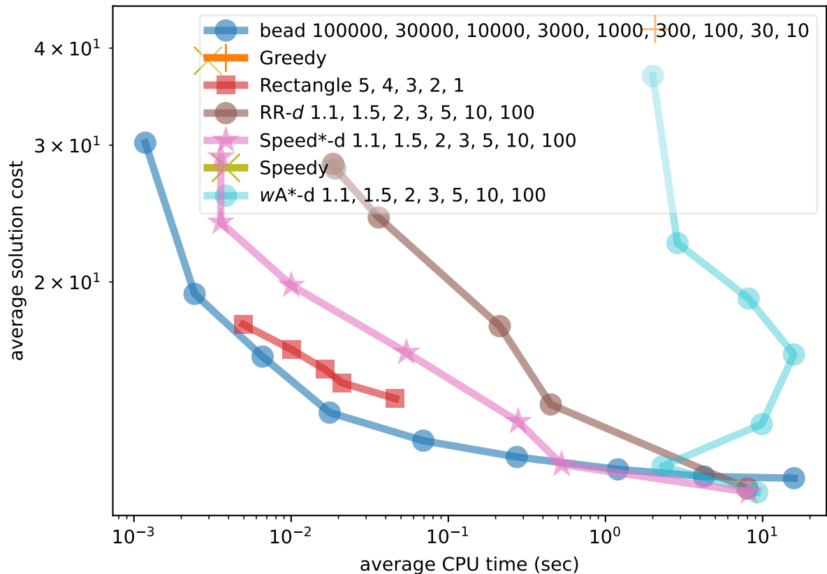
tile inverse, 54/100 commonly solved instances
