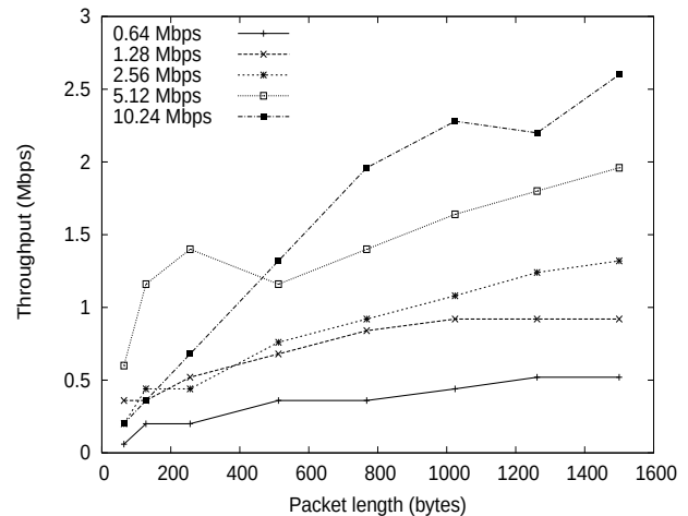
Figure 2. Experiment 1 – maximum data rate (single Broadcom-based CM, modulation format 16QAM, piggybacking and concatenation on).
