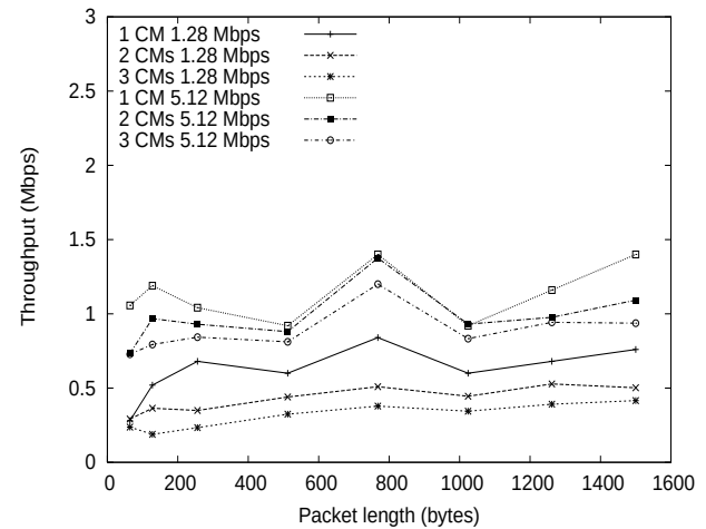
Figure 8. Experiment 4 – Per-modem throughput for one, two, and three TI-based CMs (modulation format 16QAM, piggybacking and concatenation on).
