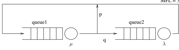
Figure 7: Closed queueing counterpart of the open feedback queue
