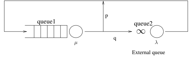
Figure 3: The feedback queue viewed as a network of two queues
