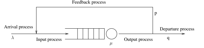
Figure 1: The M/M/1 queue with Bernoulli feedback
