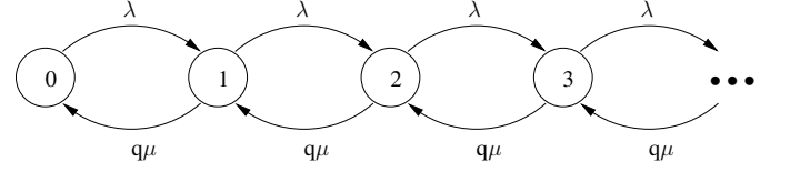
Figure 2: Markov state diagram of the feedback queue and the M/M/1 queue
