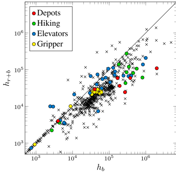
Figure 6: Number of expansions for h_b and h_{r+b} on commonly solved instances with time steps of 0.1s.
